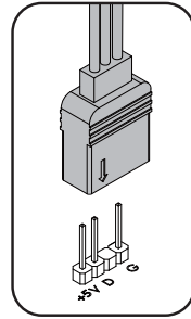
RGB connector
