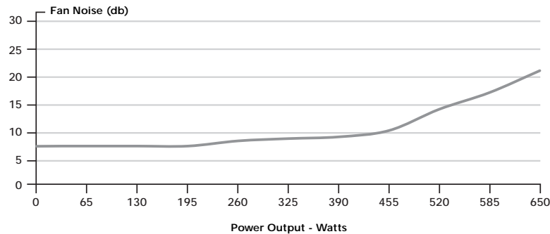
Corsair TX650M power supply fan noise curve
