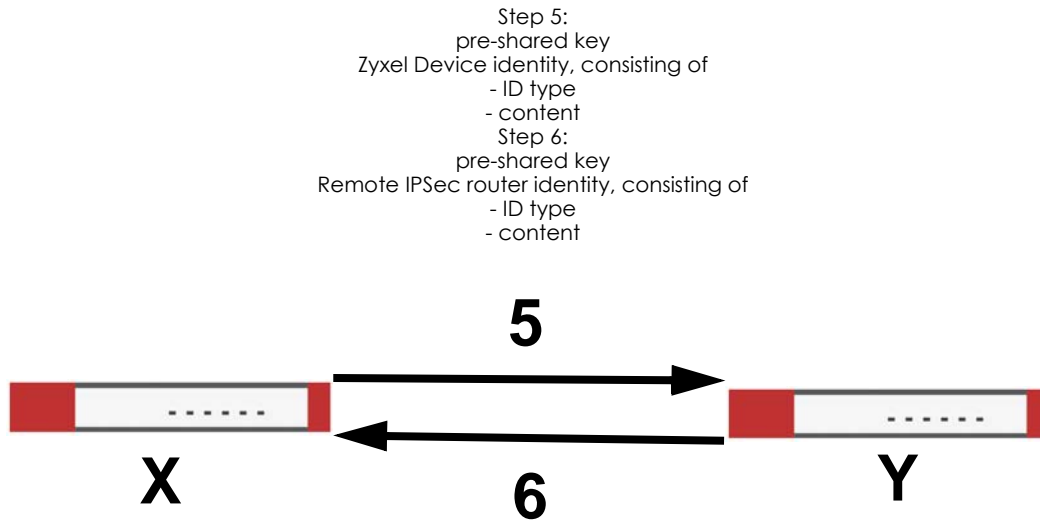
Figure 297 IKE SA: Main Negotiation Mode, Steps 5 - 6: Authentication (continued)
