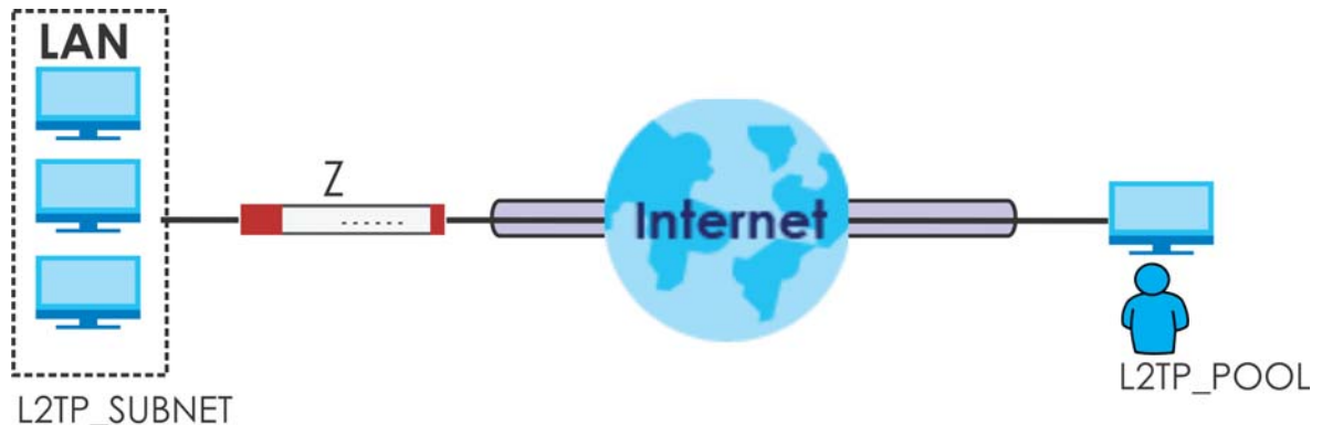
Figure 307 Policy Route for L2TP VPN
