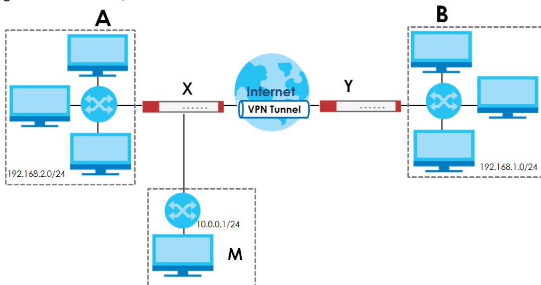
Figure 300 VPN Example: NAT for Inbound and Outbound Traffic
