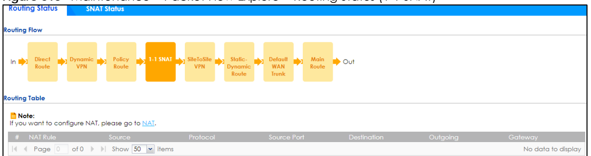
Figure 615 Maintenance > Packet Flow Explore > Routing Status (1-1 SNAT)
