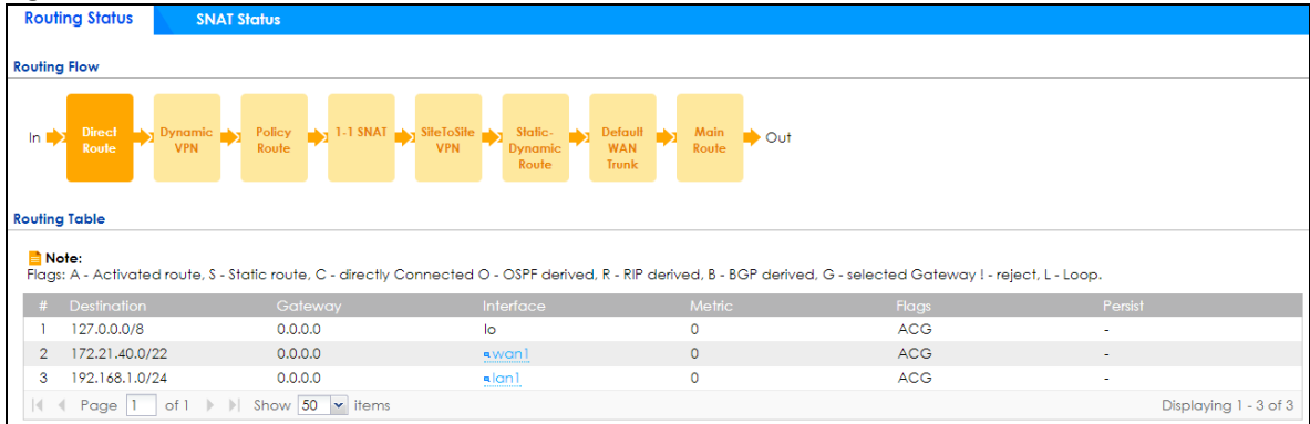
Figure 613 Maintenance > Packet Flow Explore > Routing Status (Dynamic VPN)
