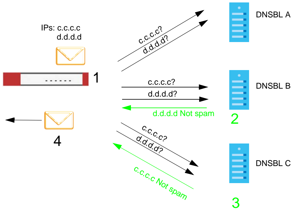
Figure 419 DNSBL Legitimate Email Detection Example
