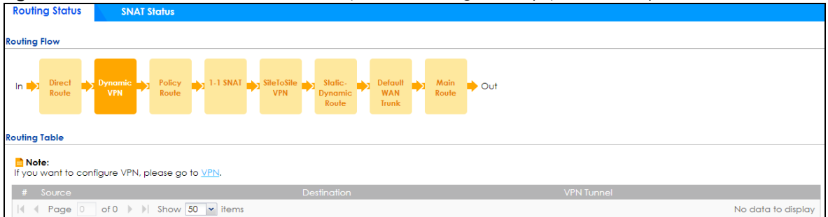
Figure 614 Maintenance > Packet Flow Explore > Routing Status (Policy Route)
