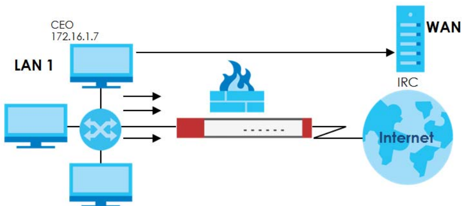
Figure 385 Limited LAN to WAN IRC Traffic Example
