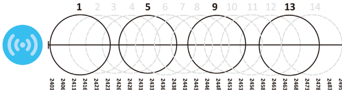
Figure 173 An Alternative Four-Channel Deployment
