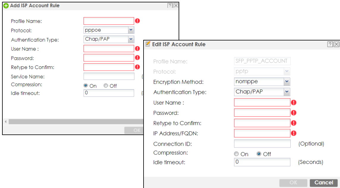
Figure 500 Configuration > Object > ISP Account > Edit
