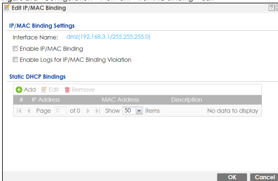
Figure 272 Configuration > Network > IP/MAC Binding > Edit
