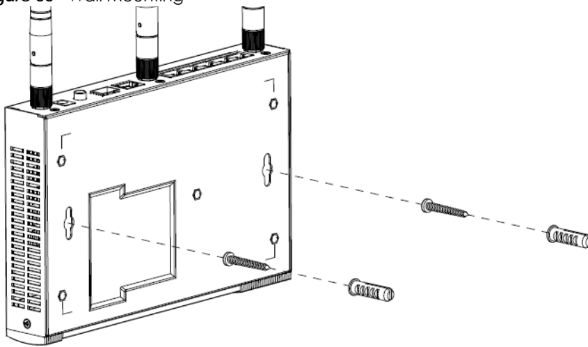
Figure 55 Wall Mounting
