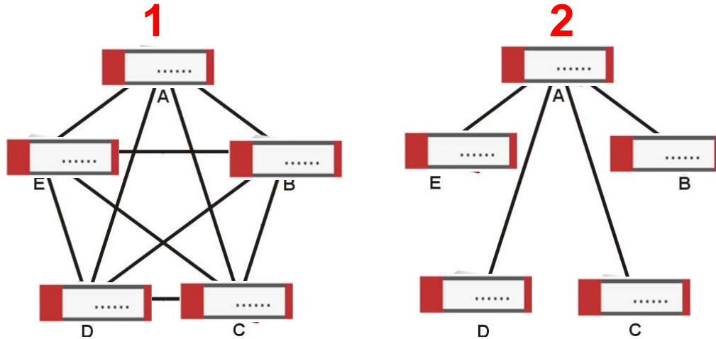
Figure 291 VPN Topologies (Fully Meshed and Hub and Spoke)
