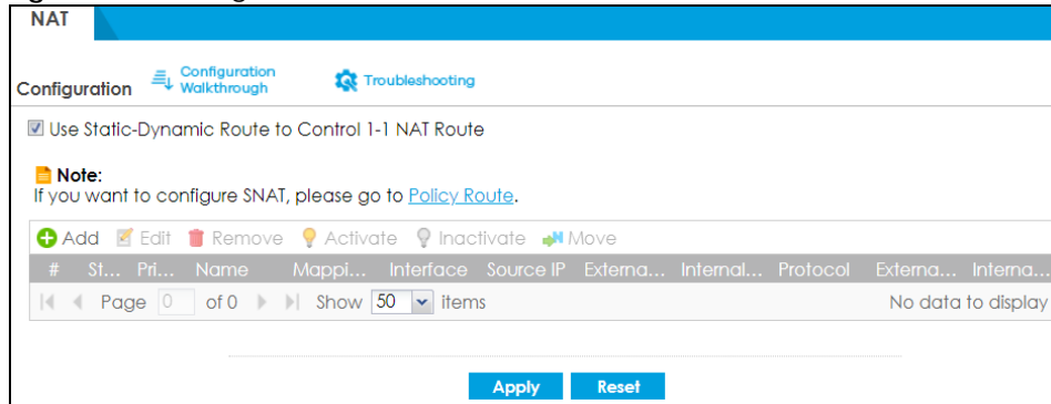
Figure 237 Configuration > Network > NAT
