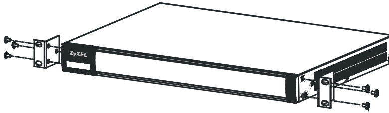
Figure 52 Attach Brackets
