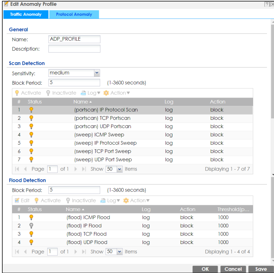
Figure 380 Configuration > Security Policy > ADP > Profile > Add-Traffic-Anomaly
