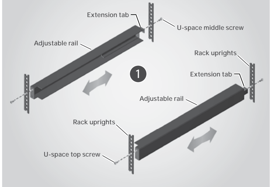
Geist SwitchAir Rack Rail Installation
