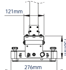
SIDE VIEW WITH CEILING PLATE TILT
