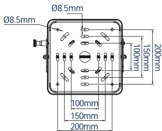
BOTTOM VIEW / INTERFACE PLATE
