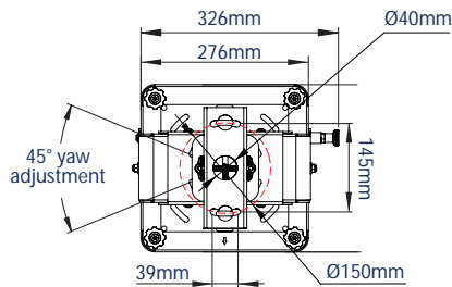
TOP VIEW / CEILING PLATE
