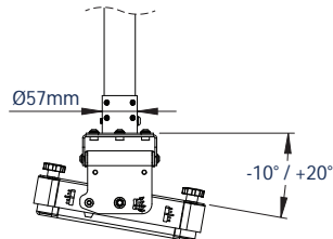
SIDE VIEW WITH INTERFACE TILT
