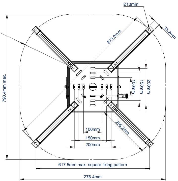
BOTTOM VIEW WITH LARGE EXTENSION LEGS
