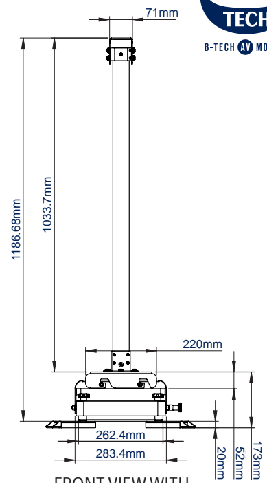
FRONT VIEW WITH EXTENSION LEGS
