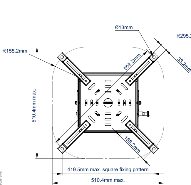
BOTTOM VIEW WITH SMALL EXTENSION LEGS
