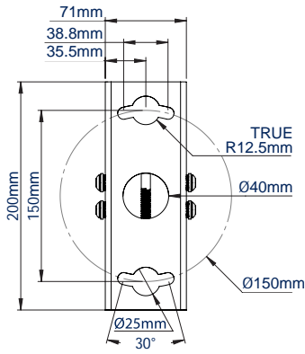
CEILING / WALL PLATE
