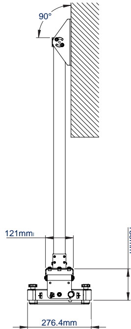
SIDE VIEW WALL MOUNTED
