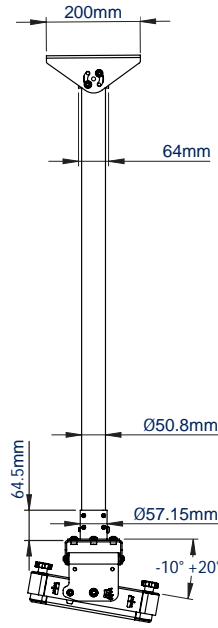
SIDE VIEW SHOWING TILT
