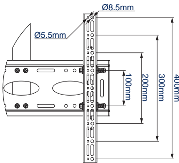
INTERFACE ARM CLOSE UP VIEW
