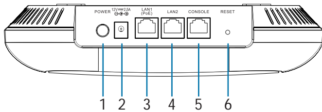
Figure 2: Rear Connectors
