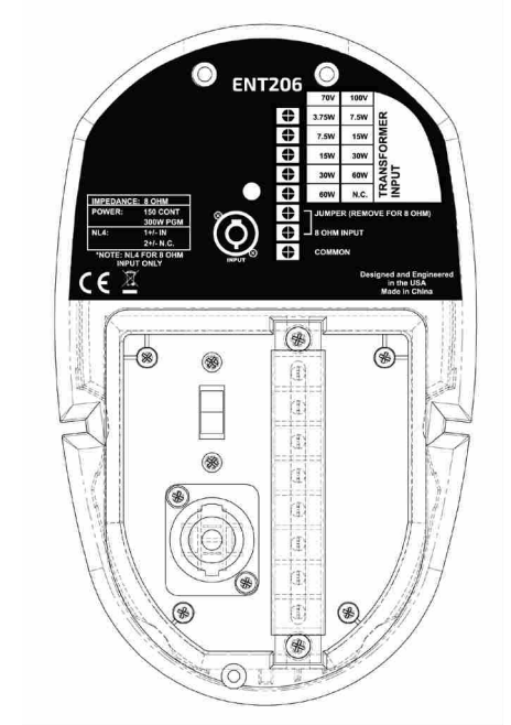
Input panel
