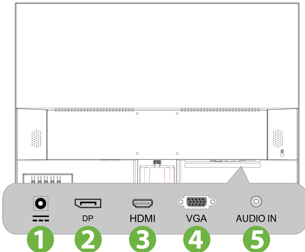
Figure.2. Connecting to a PC
