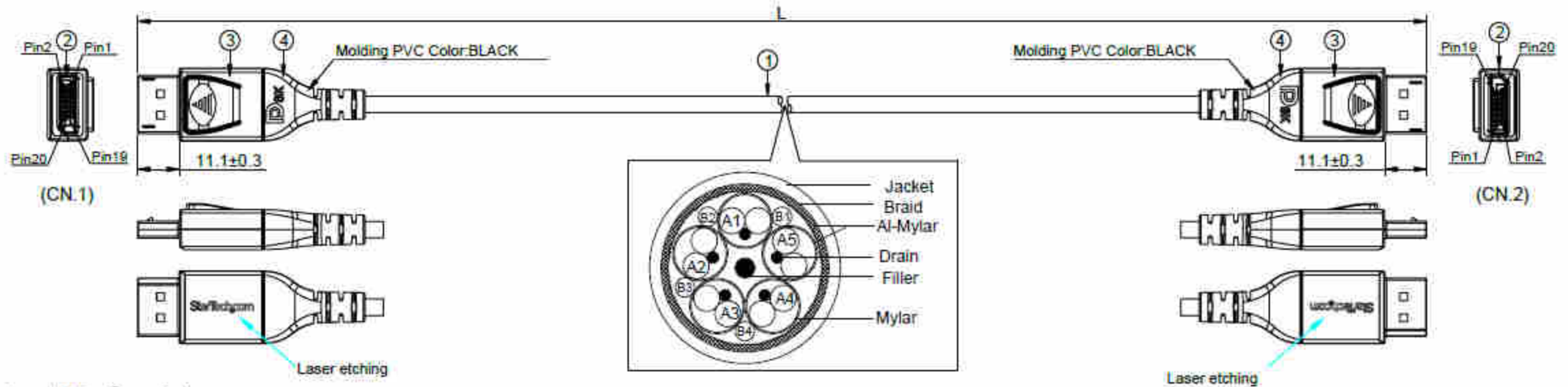
(A). Wire Pin Assignment and Wire Description.
