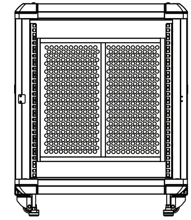
Front view (Without front door)
