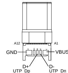
soldering view
