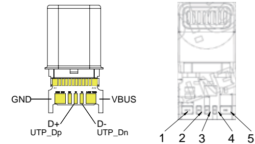
soldering view
