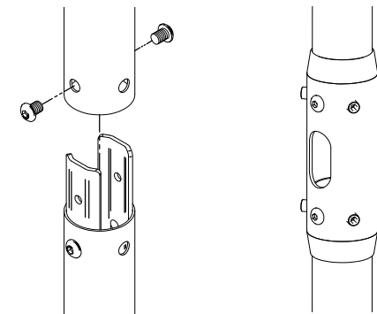
BT7823 INTERNAL POLE JOINER
