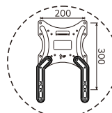
VESA 200x300
