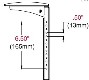
BRACKET DETAIL
