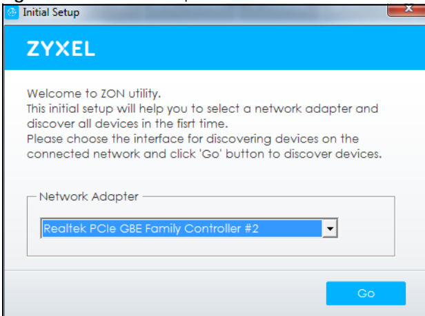
Figure 8 Network Adapter
