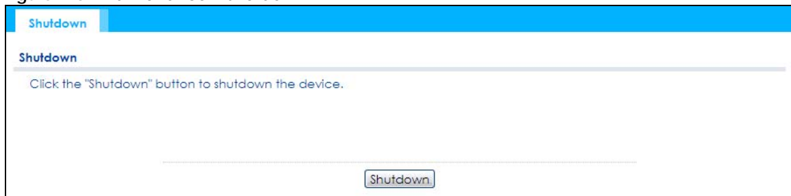
Figure 113 Maintenance > Shutdown
