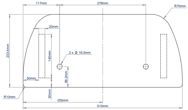
BT4002-TPC TOP VIEW
