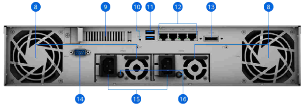
Rear (RS1221RP+)
