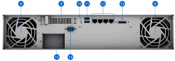
Rear (RS1221RP+)
