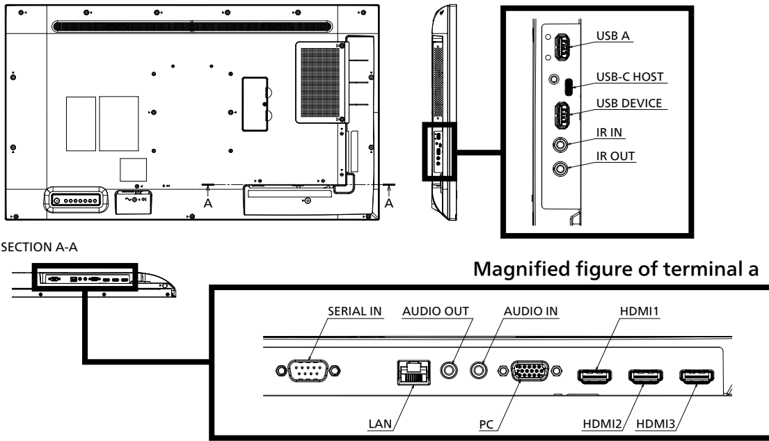
Sectional view of terminal a (SERIAL IN / LAN / AUDIO OUT / AUDIO IN / PC / HDMI 1/2/3)
