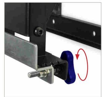
Tool-less micro-adjustment of +/-7.5mm at each corner for seamless display alignment
