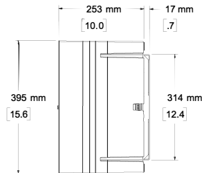
Right View
