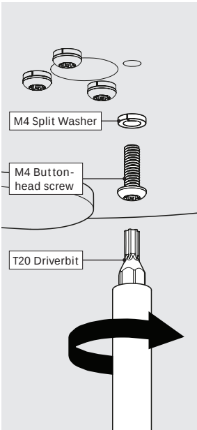
1 Attach your chosen Mounting Arm to the Freestanding Base. Ensure the correct fixings are used for your assembly.
