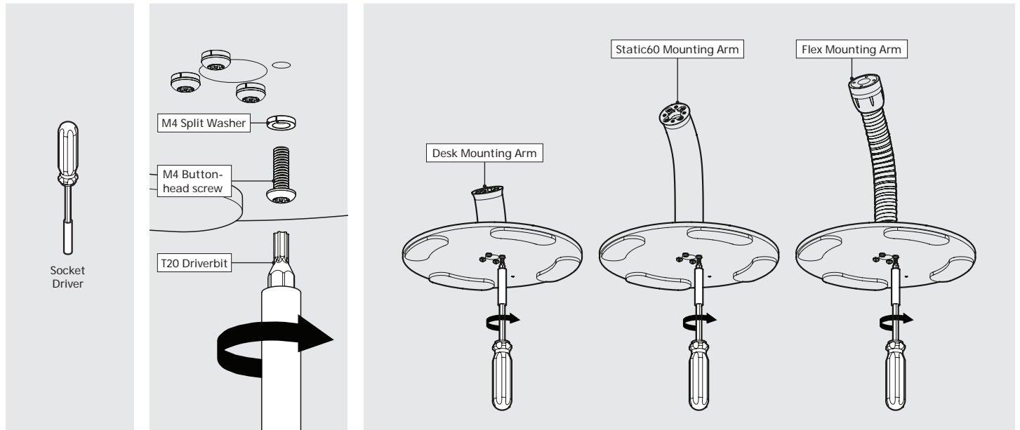
0 Tools Required 1 Attach your chosen Mounting Arm to the Freestanding Base. Ensure the correct fixings are used for your assembly.
