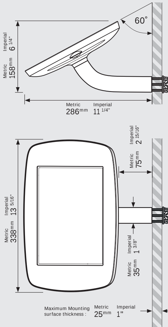
Mounting: Fixing from Below
