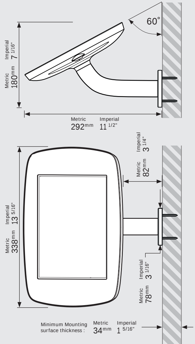
Mounting: Fixing from Above
