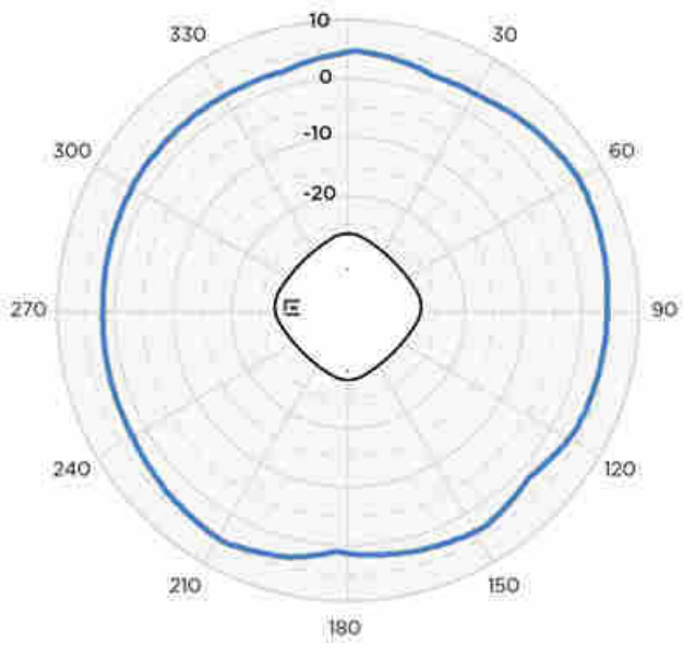
5G Azimuth
