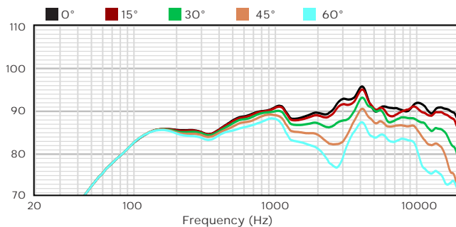
HORIZONTAL OFF-AXIS RESPONSE (dB)
