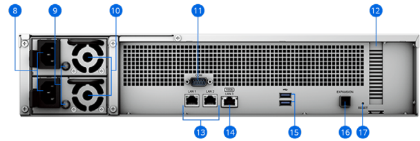
RS2423RP+ (Rear)
