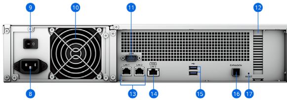
RS2423+ (Rear)
