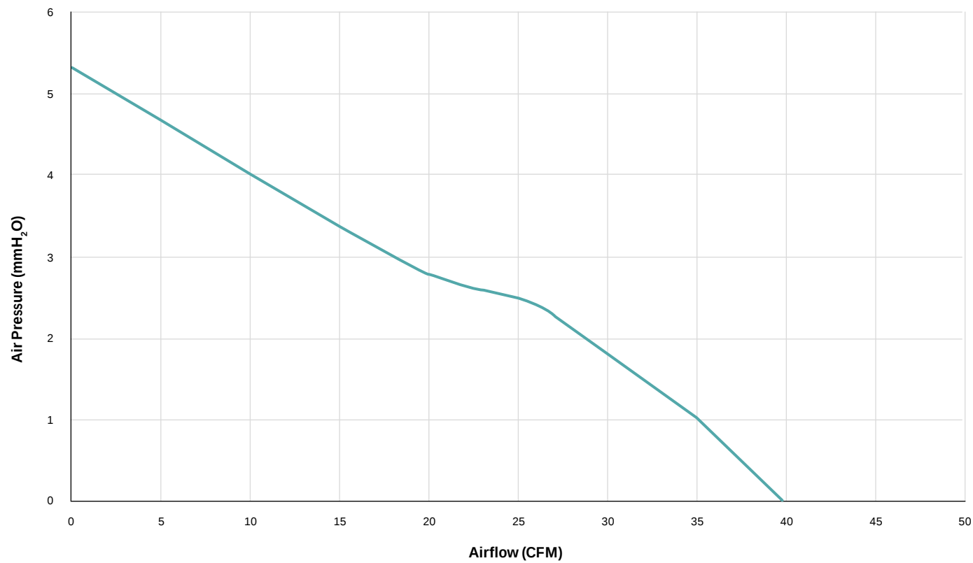
5000 rpm P-Q Curve
