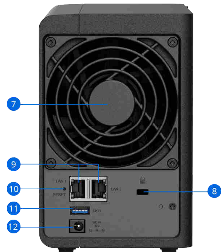
DS224+ (Rear)
