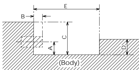
Sectional view of terminal b (AUDIO OUT R / AUDIO OUT L / USB / ANTENNA / CABLE IN / AUDIO IN / PC IN / HDMI 1)
