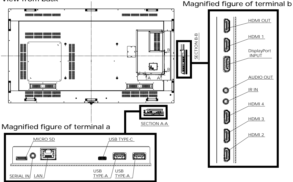
Sectional view of terminal a (MICRO SD / SERIAL IN / LAN / USB TYPE-C / USB TYPE-A / USB TYPE-A)
