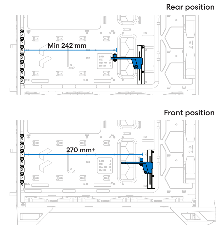
Adjusting the reach of the GPU Support Bracket
