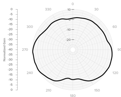
V-Plane Co-Polar
