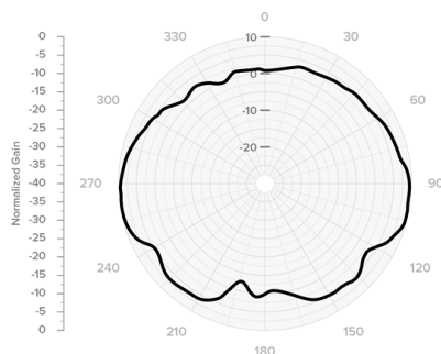
V-Plane Co-Polar
