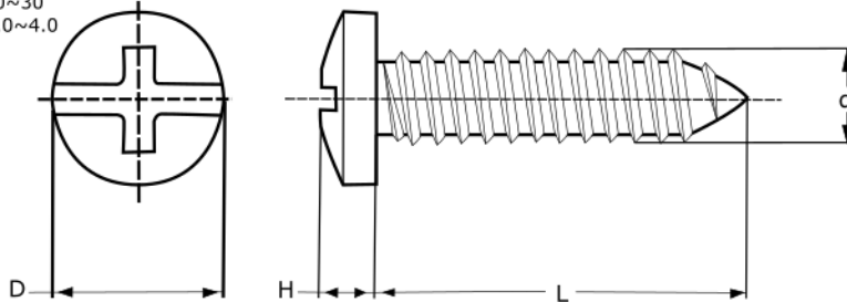
Figure 76 Wall Mounting Screw Specifications
