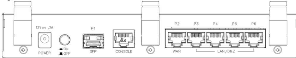
Figure 70 USG FLEX 200 Rear Panel
