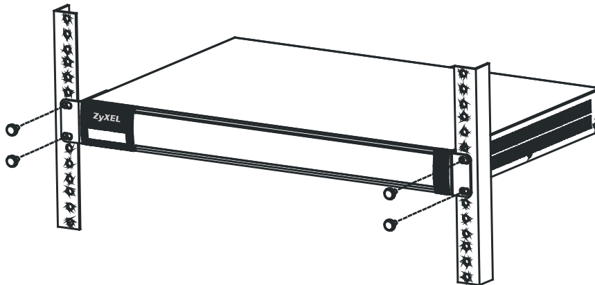
Figure 75 Mount on Rack
