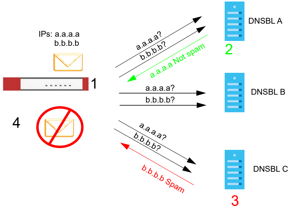
Figure 559 DNSBL Spam Detection Example
