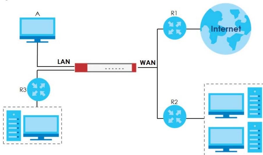
Figure 295 Example of Policy Routing Topology
