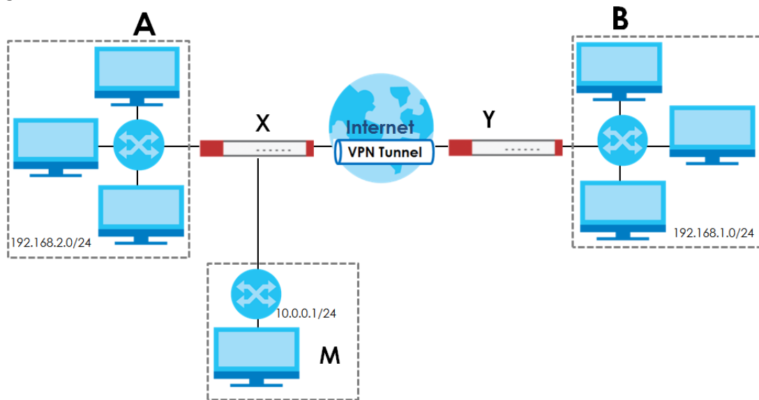
Figure 386 VPN Example: NAT for Inbound and Outbound Traffic
