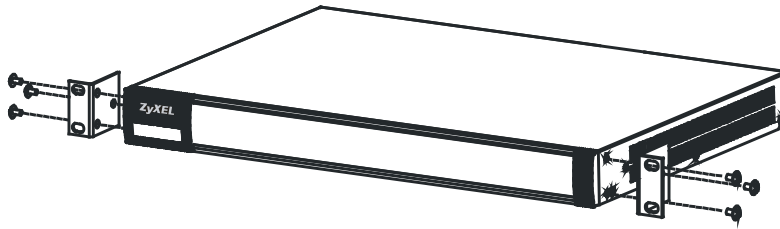
Figure 74 Attach Brackets
