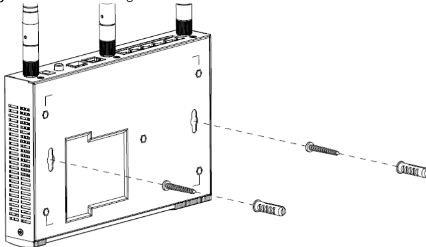
Figure 77 Wall Mounting
