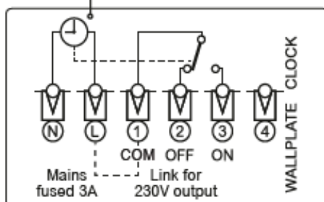
One Channel: WT714R and WV714R
