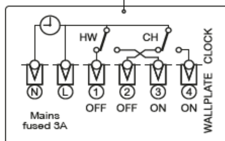
Two Channel: WT724R and WV724R
