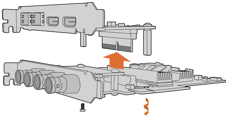
DeckLink 4K Extreme 12G's mezzanine card can easily be removed.
