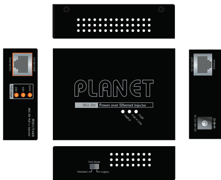
Figure 1: POE-171A-60 Outlook
