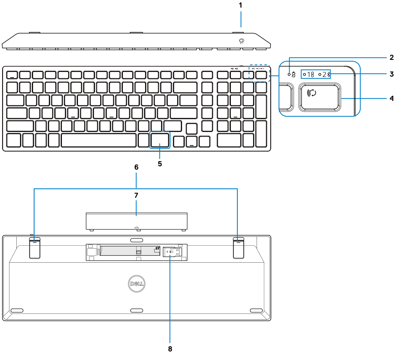
Figure 2. Keyboard features
