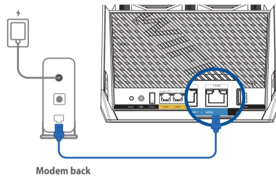
Modem back
