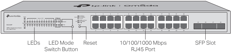
Figure 1-5 Front Panel of SG2428P
