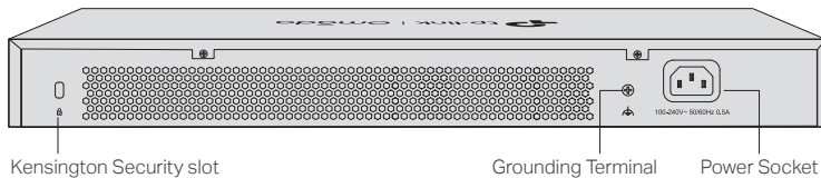
Figure 1-7 Rear Panel
