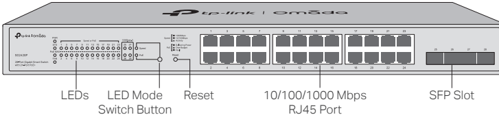
Figure 1-5 Front Panel of SG2428P
