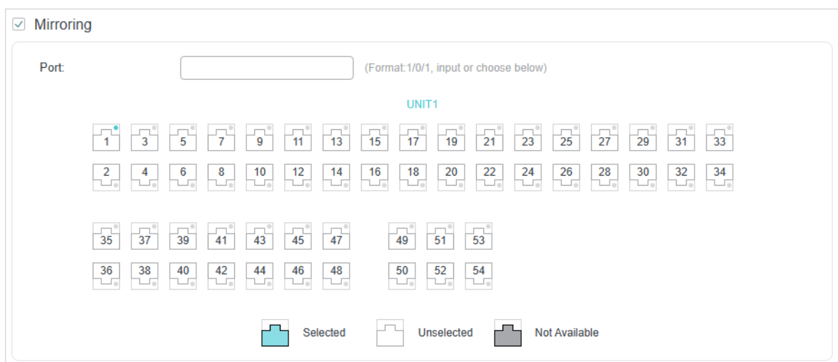
Figure 2-29 Configuring Mirroring
