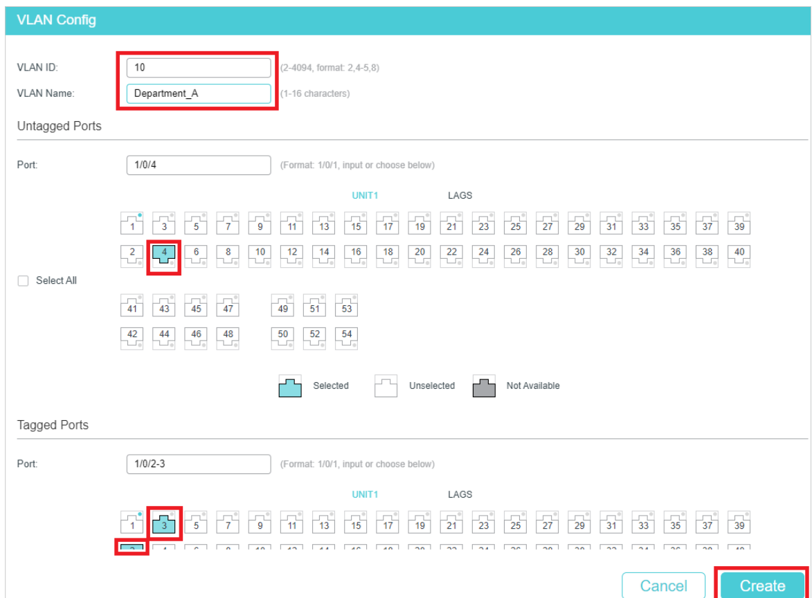
Figure 3-6 Creating VLAN 10
