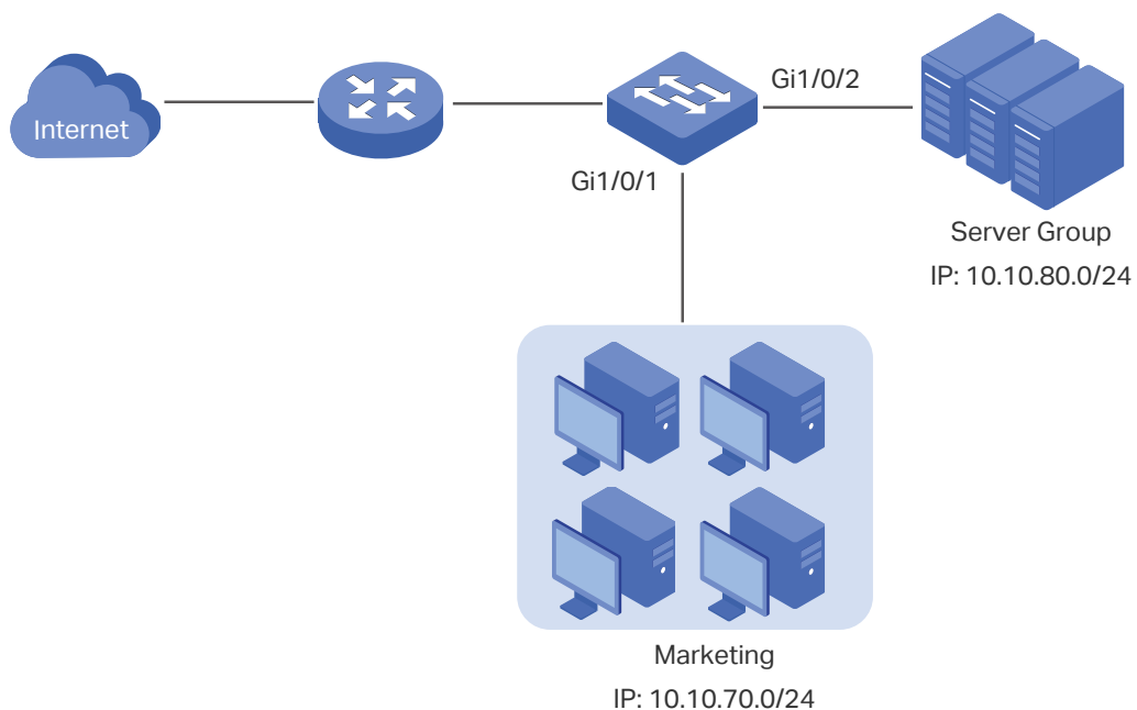
Figure 3-12 Network Topology
