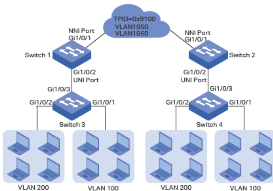
Figure 4-10 Network Topology
