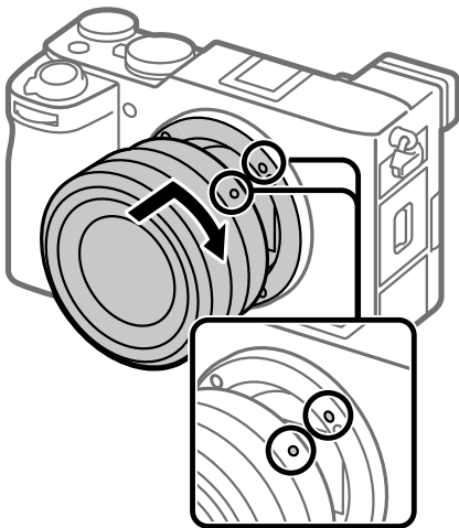
Mounting indexes
