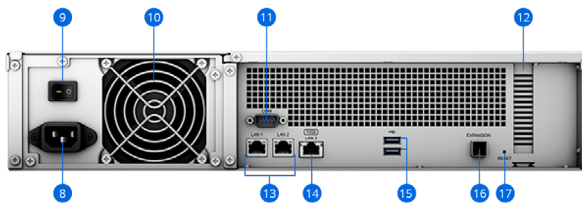
RS2423+ (Rear)
