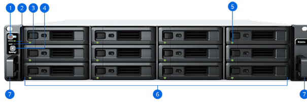
Front
