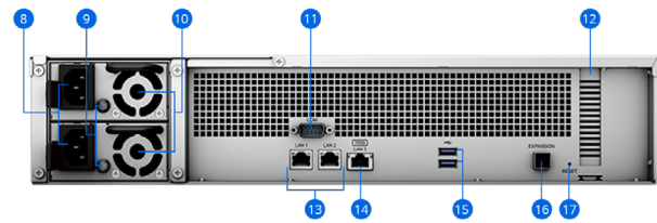
RS2423RP+ (Rear)
