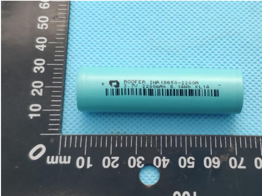
Cells /电芯 (INR18650-2200A 3.7V 2200mAh 8.14Wh)
