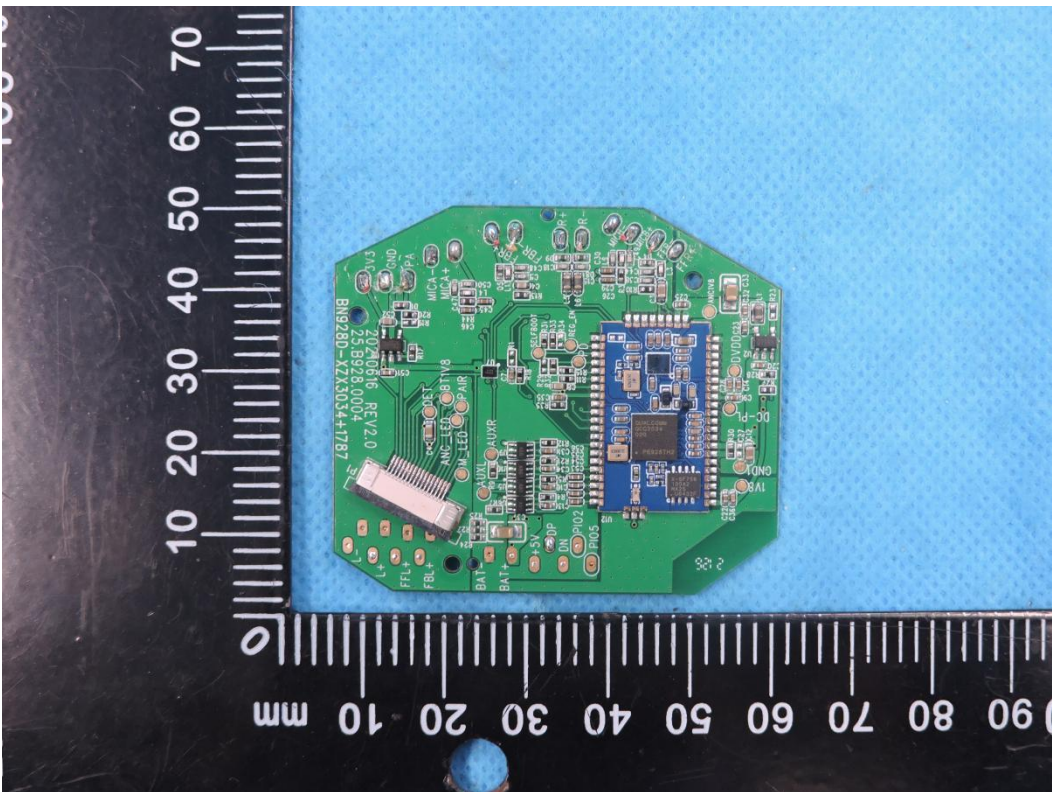
Photo 8: PCB view
