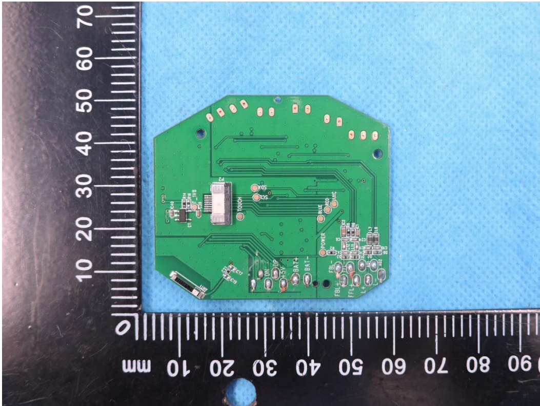
Photo 9: PCB view
